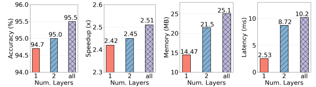
Fig. 9. Performance of ODE with different numbers of model layers for data evaluation and selection on industrial TC task.
