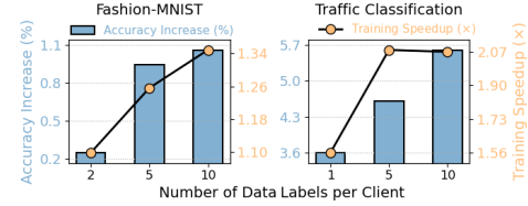
Fig. 14. Robustness of ODE-Sim to data heterogeneity.
