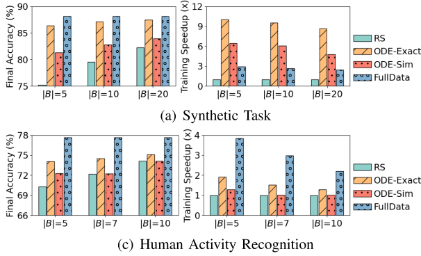
Fig. 12. Robustness of ODE to on-device storage capacities.
